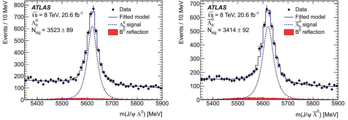
Fig. 1. The invariant mass distributions m(J/\psi \Lambda^0) (left plot) and m(J/\psi \bar{\Lambda}^0) (right plot) for selected \Lambda_b^0 and \bar{\Lambda}_b^0 candidates, respectively. The solid histograms represent the fit results (see text). The \Lambda_b^0 signals (dashed lines) and the B^0 reflections are also shown.
