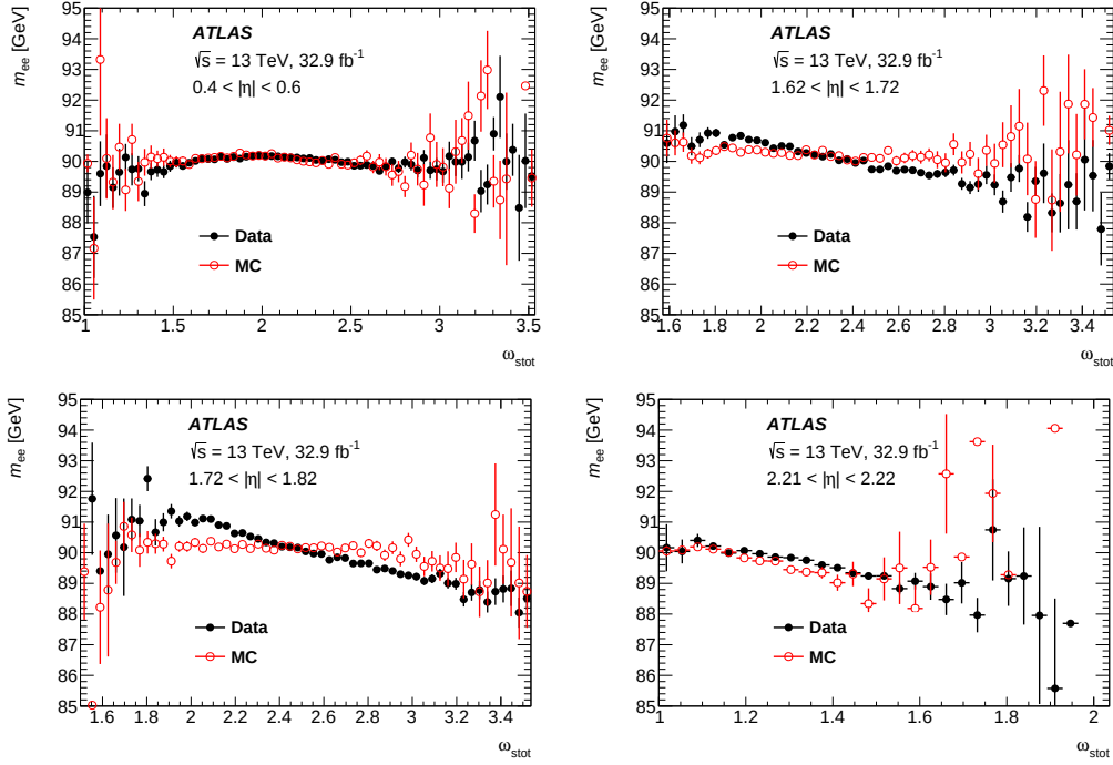
Figure 12. The mean of the dielectron mass for Z candidates ( m_{ee} ), in data and simulation, as a function of the lateral shower width ( \omega_{\text{stot}} ) for different regions in |\eta| .
