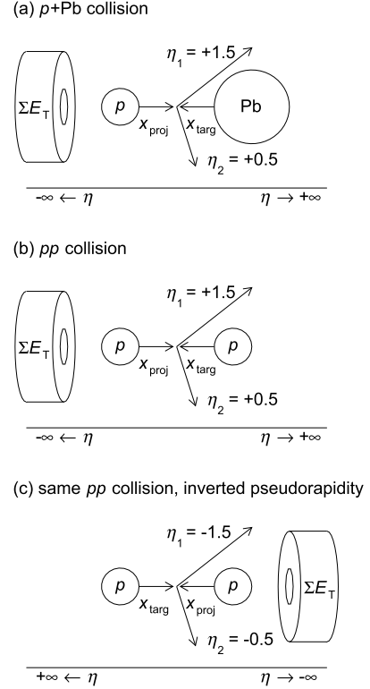
Fig. 1. Schematic illustration of the kinematic variables in the measurement. Panel (a) illustrates the convention in p + \text{Pb} collisions. Panels (b) and (c) illustrate how a single pp event provides a measurement of \sum E_T at two values of \eta^{\text{dijet}} = (\eta_1 + \eta_2)/2 , in this case for \eta^{\text{dijet}} = +1 and for \eta^{\text{dijet}} = -1 , respectively.
