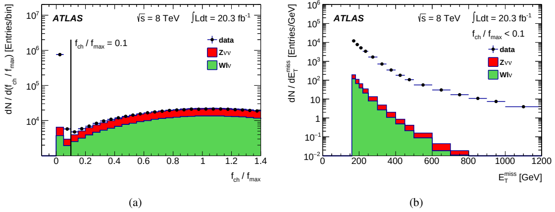
Figure 18. The distribution of the ratio f_{\text{ch}}/f_{\text{max}} for leading jets in the events from colliding bunches triggered by the E_{\text{T}}^{\text{miss}} trigger with an offline requirement of E_{\text{T}}^{\text{miss}} > 160 GeV (a). The value f_{\text{ch}}/f_{\text{max}} = 0.1 , used to separate NCB from pp collision processes, is indicated by the black line. The E_{\text{T}}^{\text{miss}} distribution for the NCB events determined by the f_{\text{ch}}/f_{\text{max}} < 0.1 selection (b). Data is compared to the Standard Model expectation from the Z \rightarrow \nu\nu + \text{jets} and W \rightarrow l\nu + \text{jets} electroweak processes. Other pp collision products, such as top and dibosons, that contribute to the total expectation by less than approximately 10% over the whole E_{\text{T}}^{\text{miss}} spectrum are not shown.
