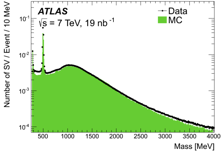
Figure 3. Invariant-mass spectrum of the reconstructed secondary vertices, assuming the pion mass for all tracks, in data (points) and MC simulation (solid histogram).
