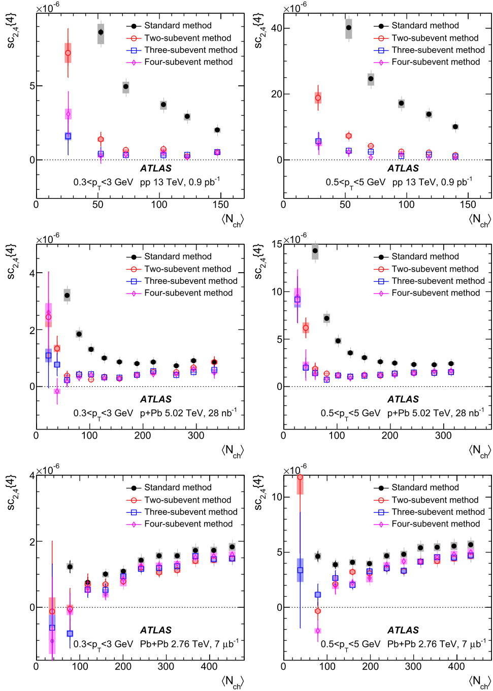
Fig. 2. The symmetric cumulant sc_{2,4}\{4\} as a function of \langle N_{ch} \rangle for 0.3 < p_T < 3 \text{ GeV} (left panels) and 0.5 < p_T < 5 \text{ GeV} (right panels) obtained for pp collisions (top row), p\text{+Pb} collisions (middle row) and low-multiplicity \text{Pb+Pb} collisions (bottom row). In each panel, the sc_{2,4}\{4\} is obtained from the standard method (filled symbol), two-subevent method (open circles), three-subevent method (open squares) and four-subevent method (open diamonds). The error bars and shaded boxes represent the statistical and systematic uncertainties, respectively.
