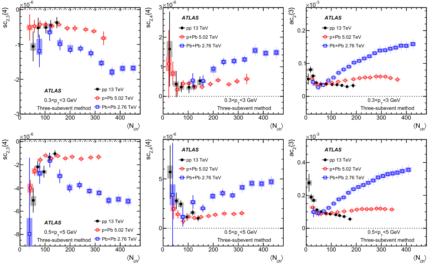
Fig. 4. The \langle N_{\text{ch}} \rangle dependence of sc_{2,3}\{4\} (left panels), sc_{2,4}\{4\} (middle panels) and ac_2\{3\} (right panels) in 0.3 < p_T < 3 GeV (top row) and 0.5 < p_T < 5 GeV (bottom row) obtained for pp collisions (solid circles), p +Pb collisions (open circles) and low-multiplicity Pb+Pb collisions (open squares). The error bars and shaded boxes represent the statistical and systematic uncertainties, respectively.
