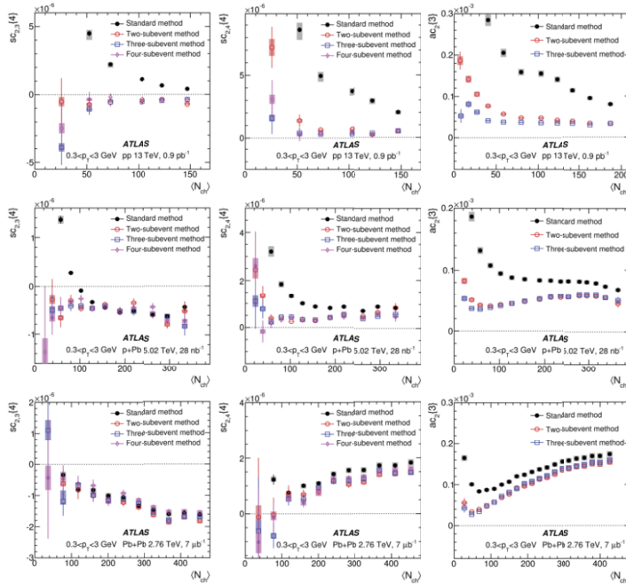
Fig. 1. The symmetric cumulants sc_{2,3}\{4\} (left column), sc_{2,4}\{4\} (middle column) and asymmetric cumulant ac_2\{3\} (right column) as a function of \langle N_{ch} \rangle obtained for pp collisions (top row), p+Pb collisions (middle row) and low-multiplicity Pb+Pb collisions (bottom row) [9]. In each panel, the results are obtained from the standard method (filled symbols), the two-subevent method (open circles), three-subevent method (open squares) and in the case of symmetric cumulants four-subevent method (open diamonds). The error bars and shaded boxes represent the statistical and systematic uncertainties, respectively.
