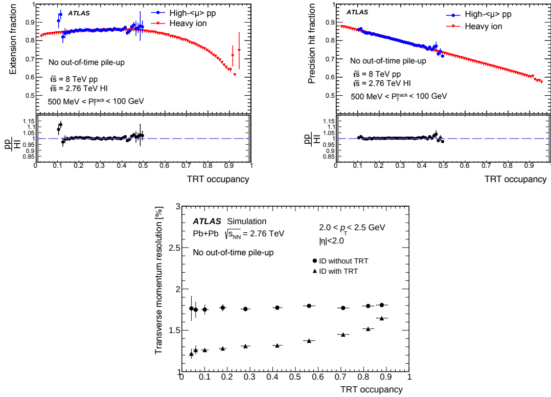
Figure 19. The TRT track extension fraction (top left), and the precision hit fraction (top right), as a function of the total TRT occupancy from minimum-bias events with 40 \leq \langle\mu\rangle \leq 70 for pp and heavy-ion collision events during the 2011–2012 operation with a Xe-based gas mixture. The p_T resolution of ID tracks as a function of the TRT occupancy (bottom) with (triangle marker) and without (circle marker) TRT measurements for heavy-ion simulations with a Xe-based gas mixture. Tracks with TRT measurements correspond to 70% of the tracks in the ID in such high-occupancy conditions as shown in the top left panel.
